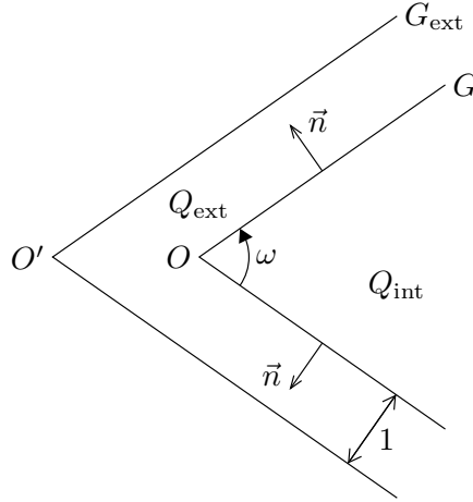
Figure 2: The infinite domain Q .
