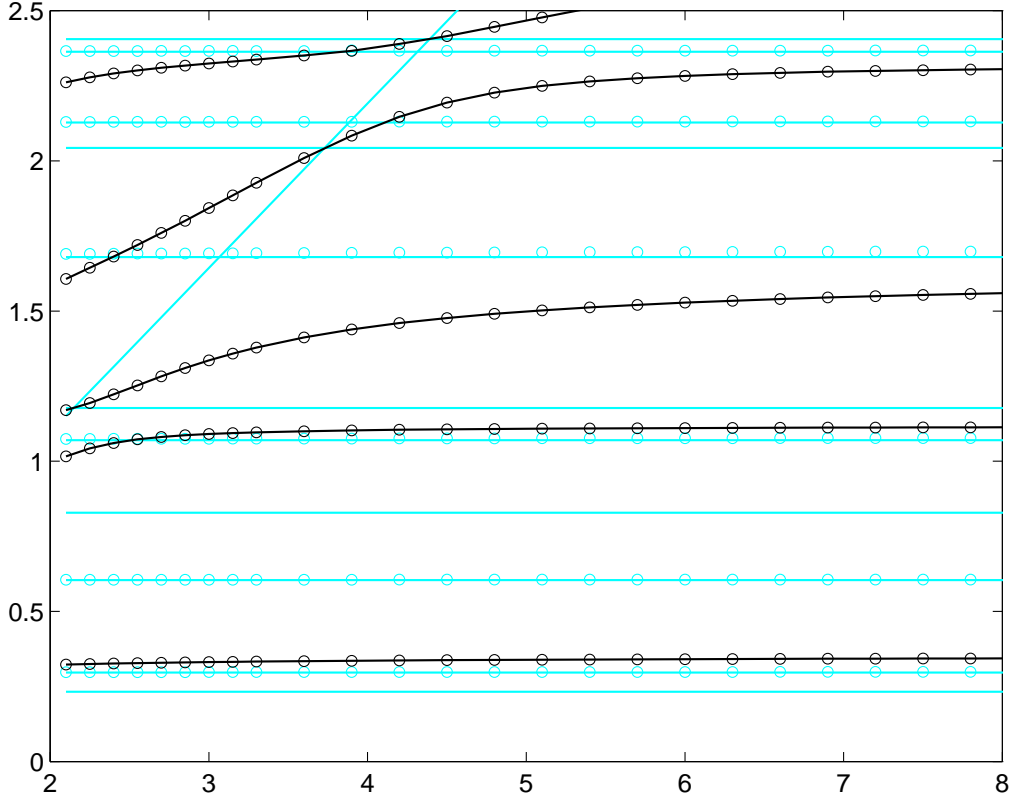
Figure 1: Lowest eigenvalues (symmetric domain)
