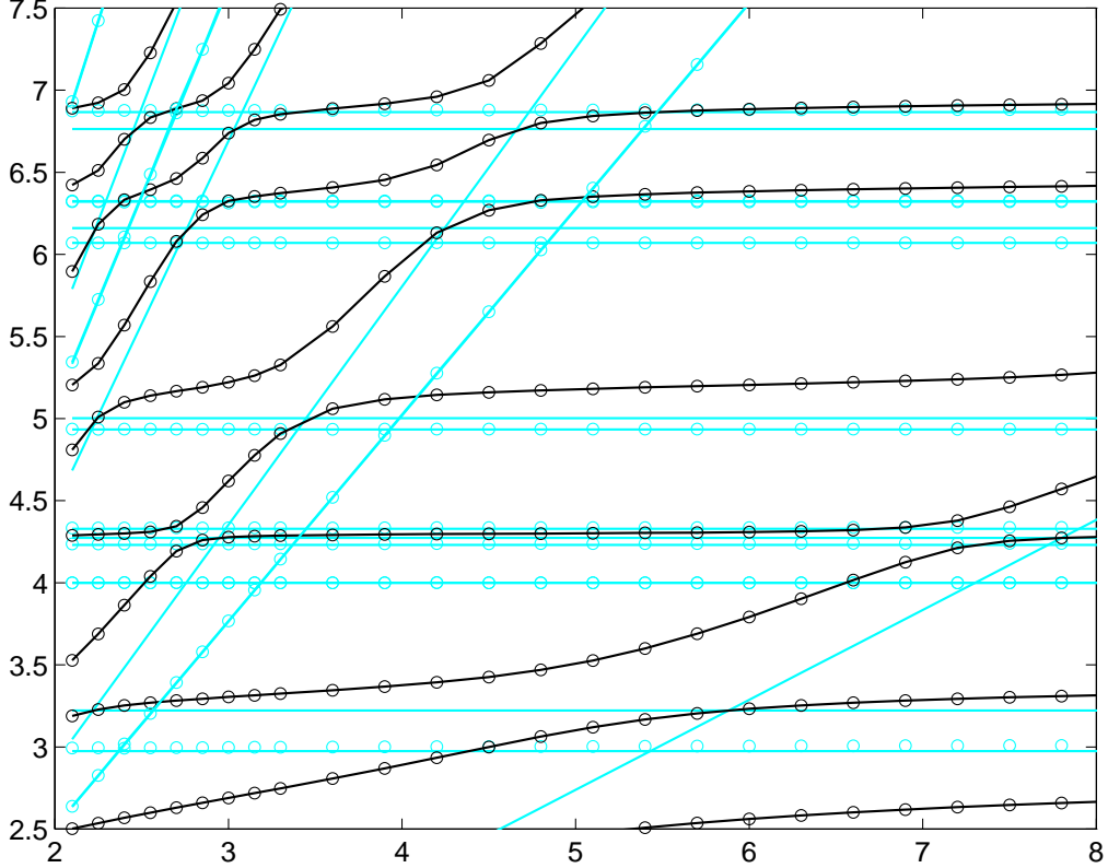
Figure 2: Further eigenvalues (symmetric domain)
